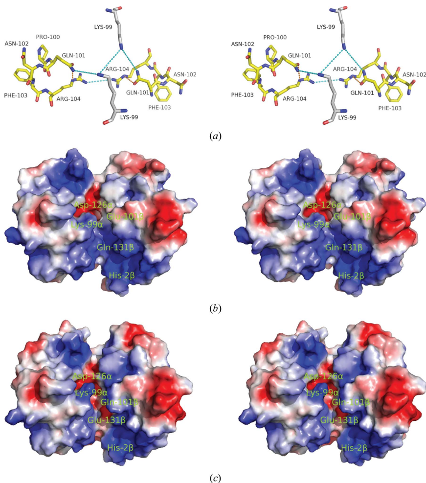
Figure 4 (a) A stereoview of the central cavity of deoxy woolly mammoth Hb. C atoms of the \alpha subunit are coloured white and C atoms of the \beta/\delta subunit are coloured yellow. Orange dotted lines indicate distances of between 3 and 4 Å in length and light blue dotted lines indicate distances of between 4 and 7.2 Å in length. In human HbA, the charge on the pairs of lysine and arginine residues is partly countered by Glu \beta/\delta 101. (b) A stereoview of the molecular surface of one \alpha\beta dimer of deoxy human HbA coloured by electrostatic potential (red, negative; blue, positive). Colour saturation corresponds to an electron energy of \pm 3kT . The \alpha chain is on the left; the central cavity is shown running vertically and the DPG binding site is at the bottom. Asp \alpha 126 is responsible for the negatively charged pocket between the two subunits and Lys \alpha 99 projects from the \alpha subunit towards Glu \beta 101. The surface potential was calculated using APBS (Baker et al. , 2001). (c) A similar figure to (b) but showing deoxy woolly mammoth Hb. The electrostatic potential is altered from the normal pattern by two mutations: Glu \beta/\delta 101 \rightarrow Gln and Gln \beta/\delta 131 \rightarrow Glu. The potential is essentially unchanged around Asn \alpha 131 and Val \beta/\delta 1, which are the sites of chloride binding in other animal Hbs. Lys \alpha 99 shows a higher potential in woolly mammoth Hb than in HbA.
